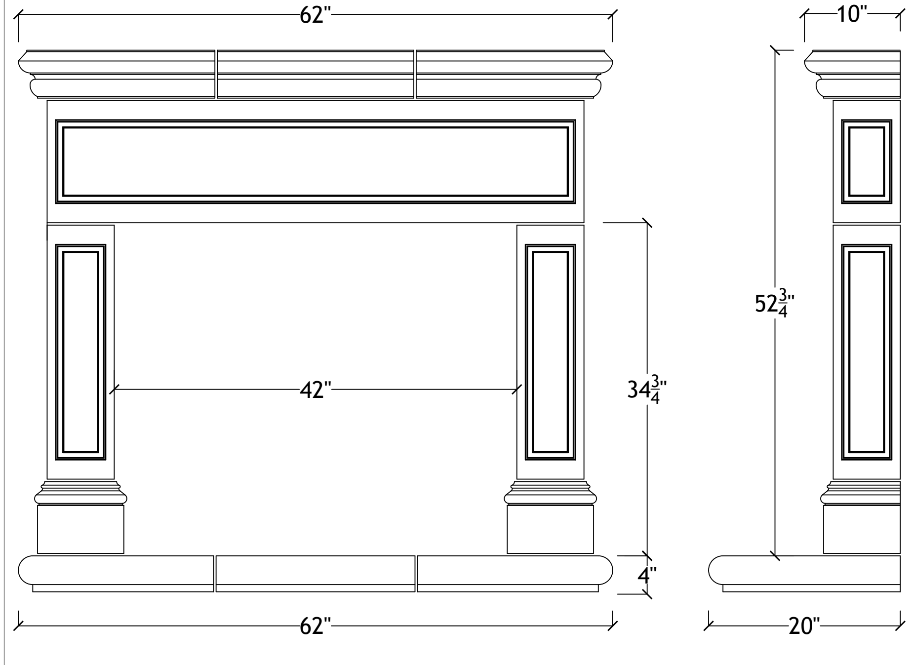
42" Devon with bullnosed hearth
