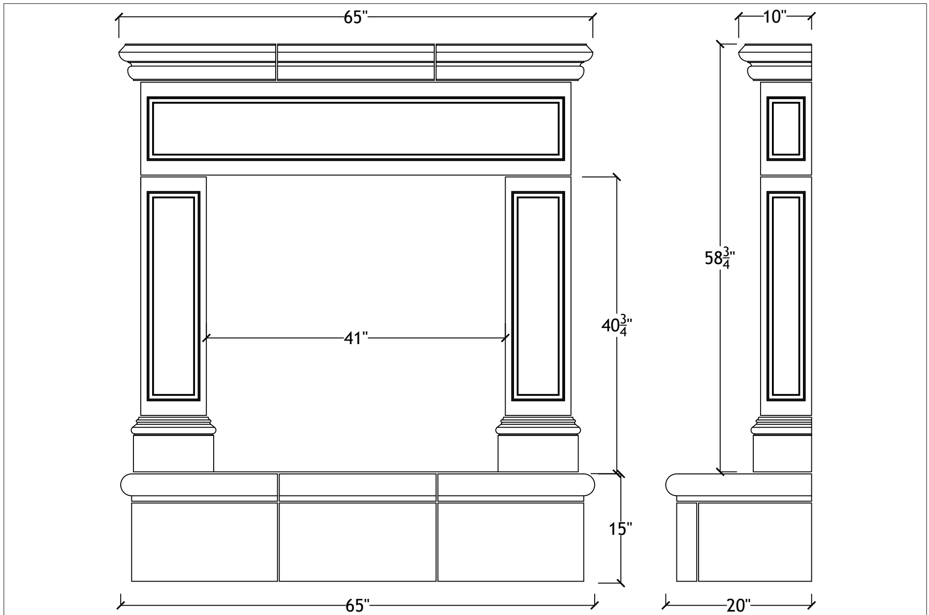
41" Devon with raised bullnosed hearth
