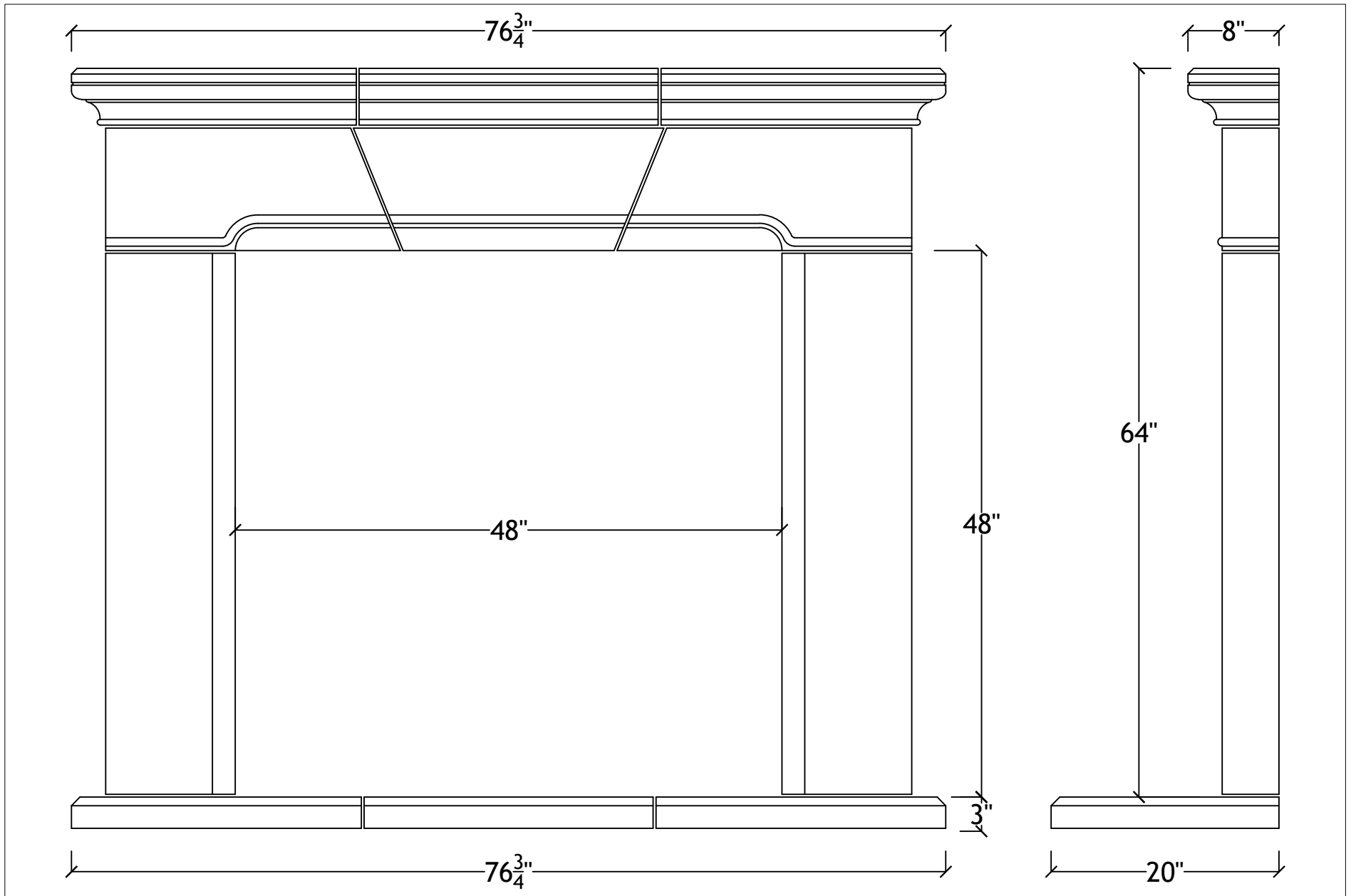
48" Conrad with hearth
