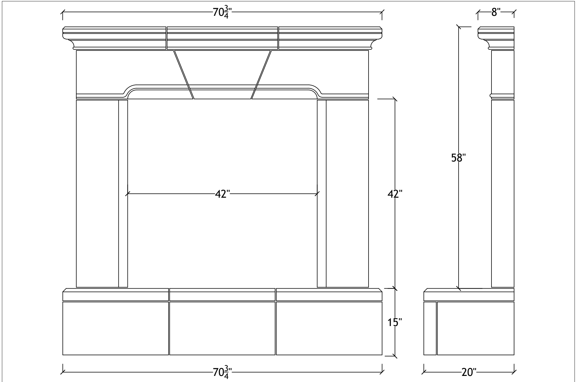
42" Conrad with raised hearth
