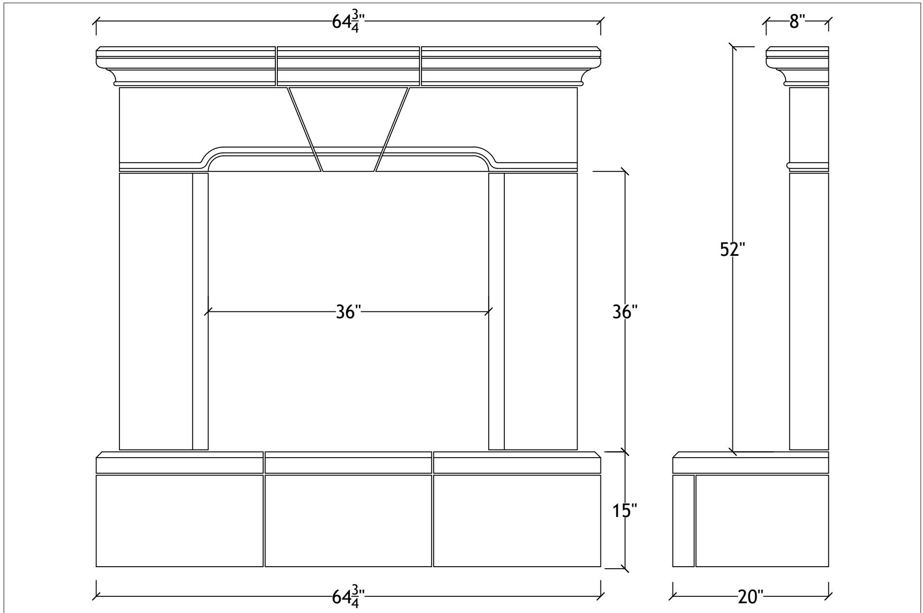
36" Conrad with raised hearth
