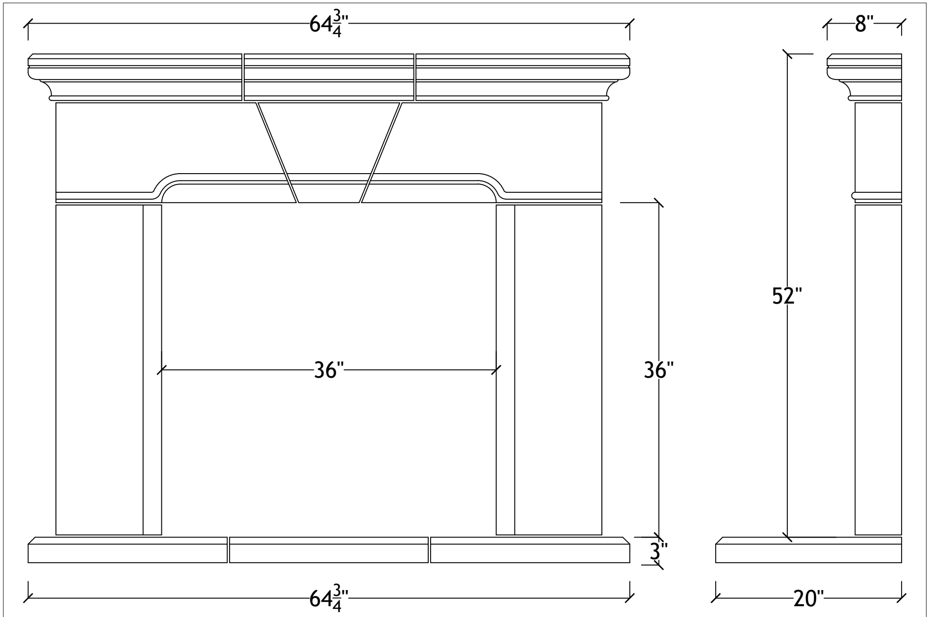
36" Conrad with hearth
