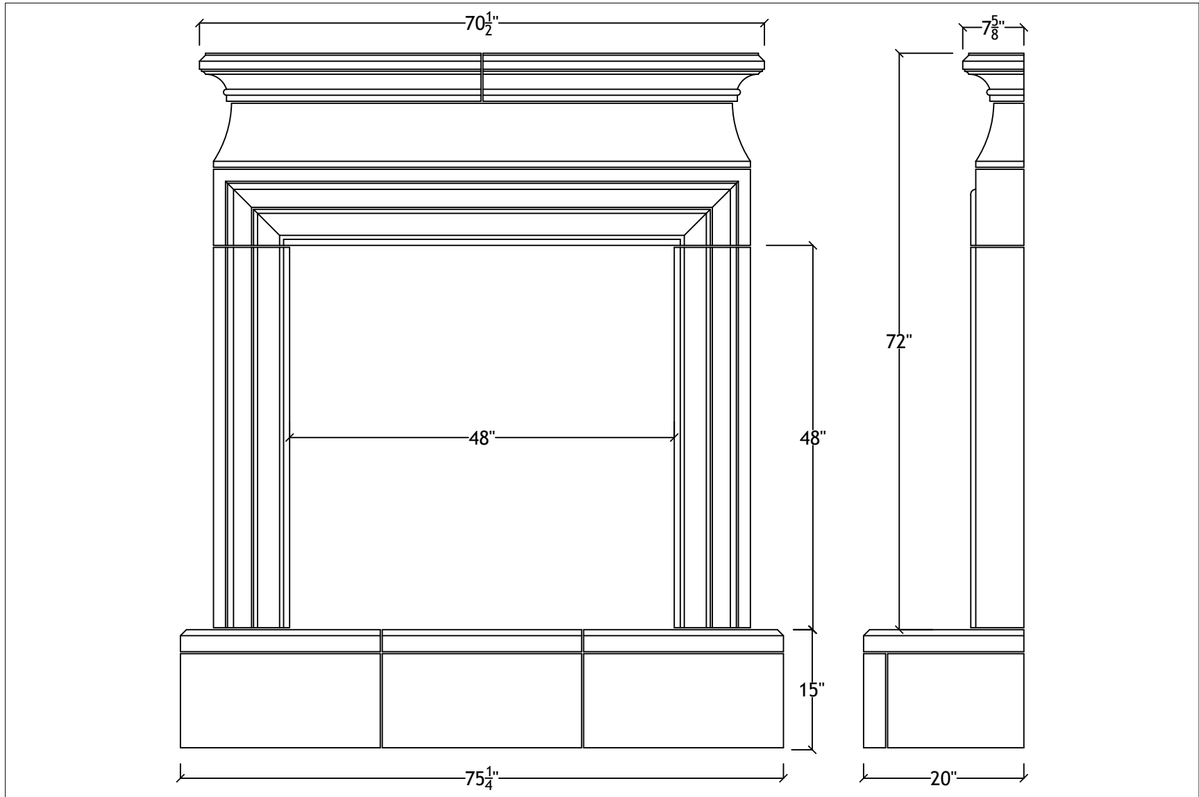
48" Chelsea with raised hearth
