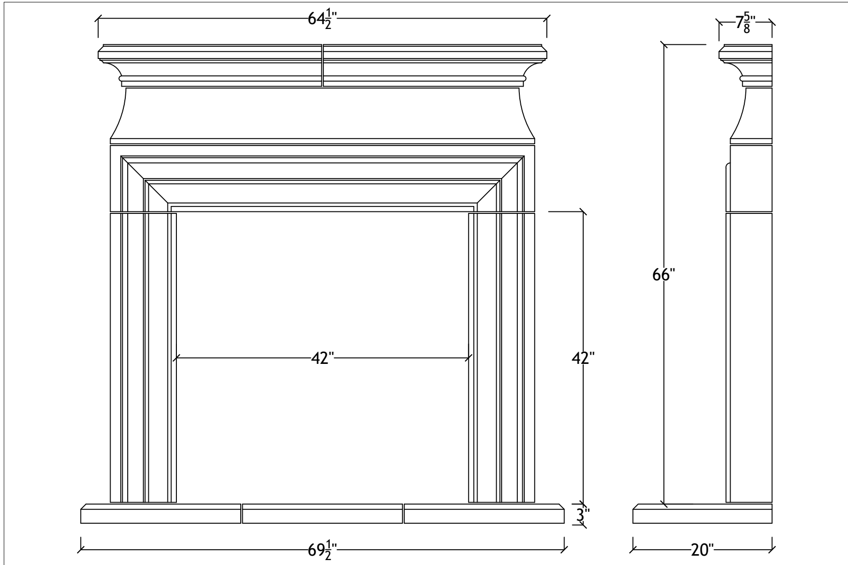
42" Chelsea with hearth
