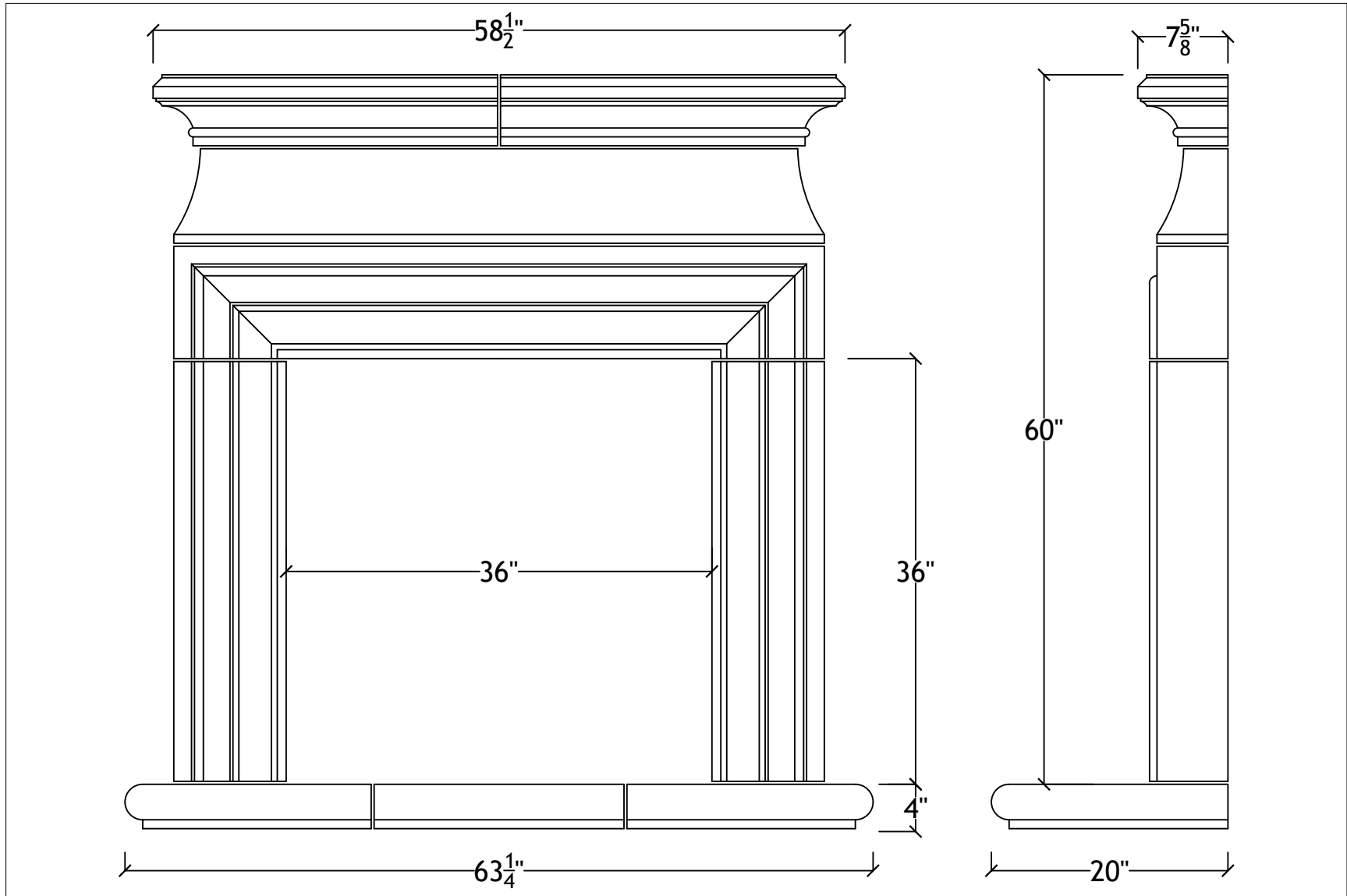
36" Chelsea with bullnosed hearth
