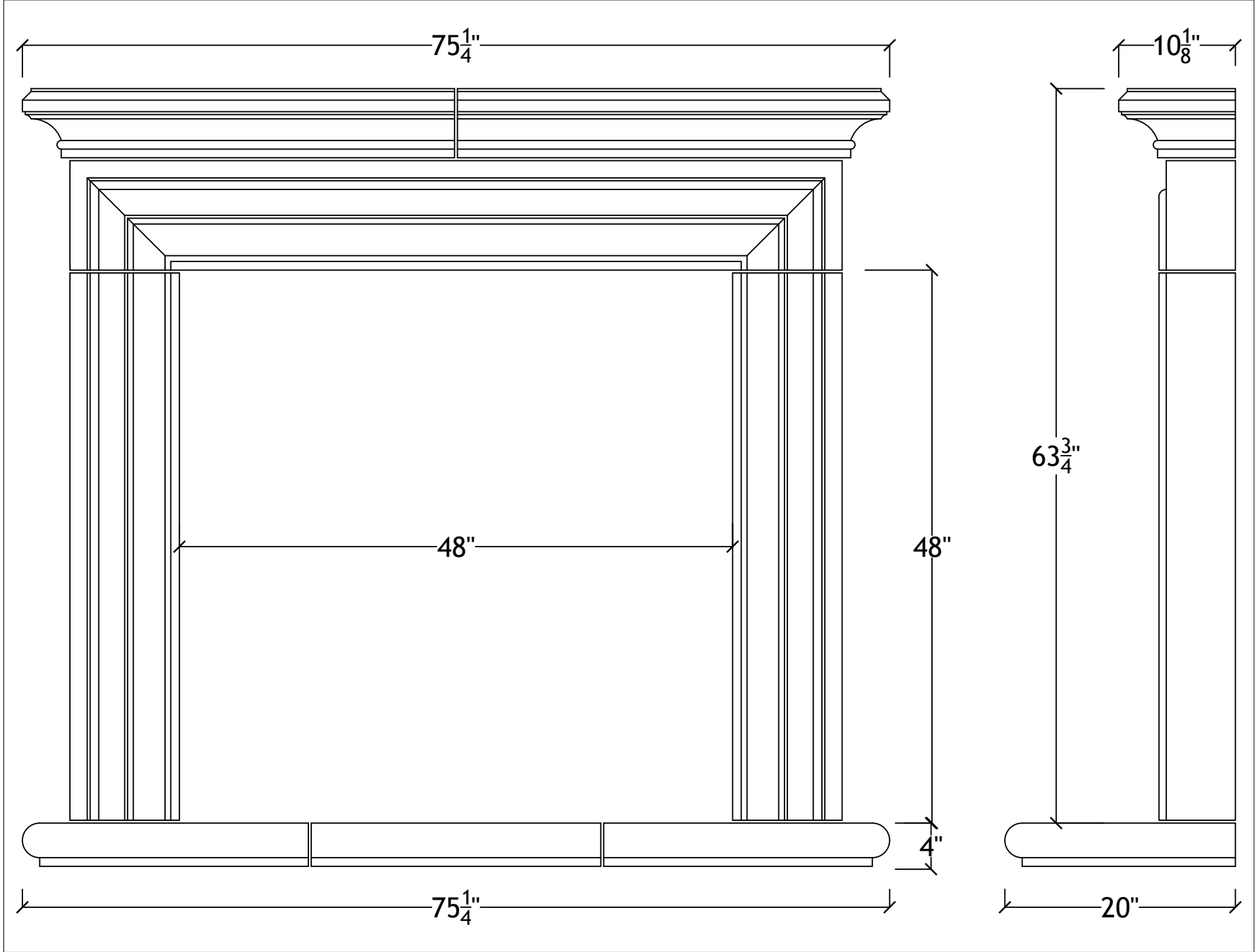
A 1 48" Capri with bullnosed hearth
