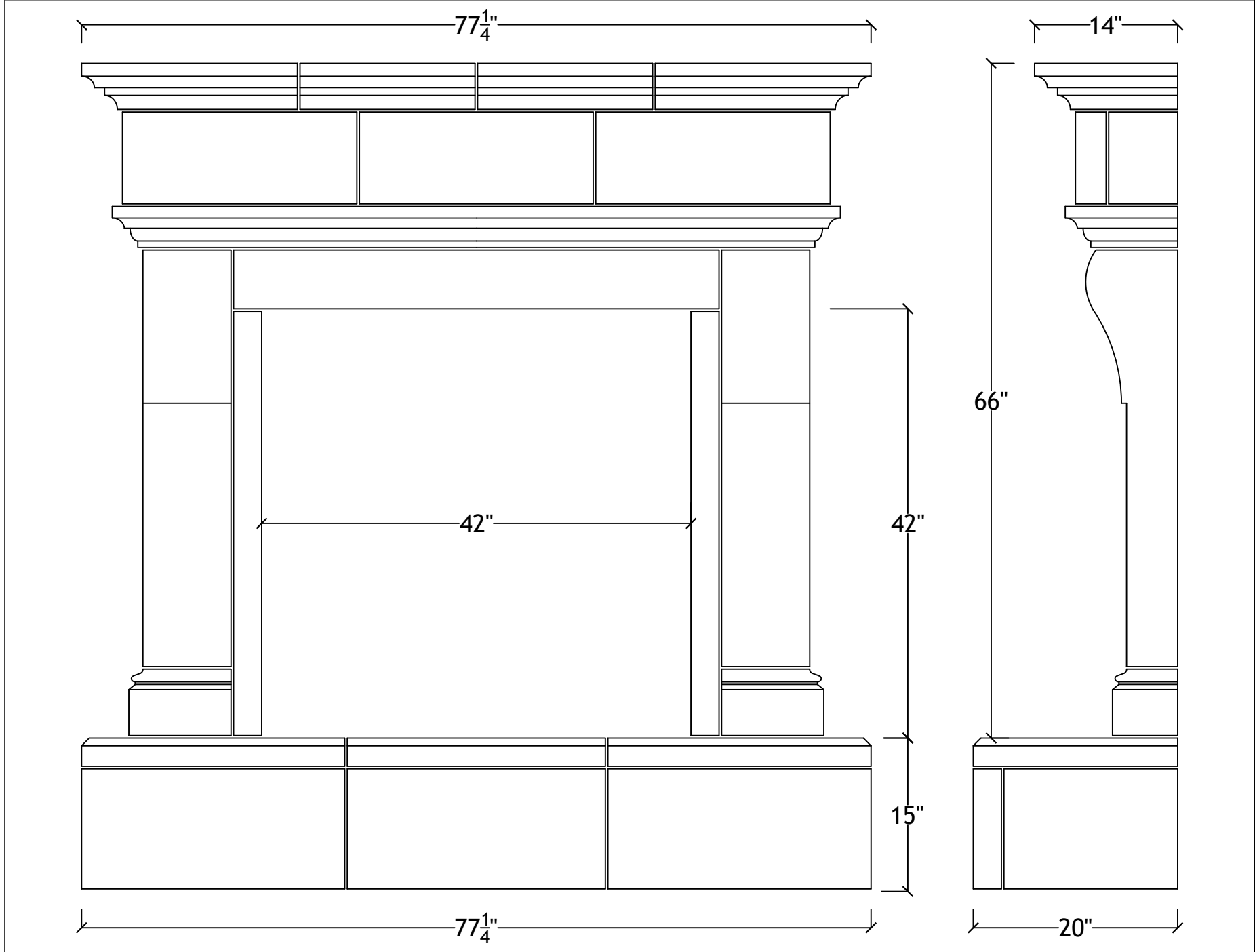
42" Cambridge with raised hearth
