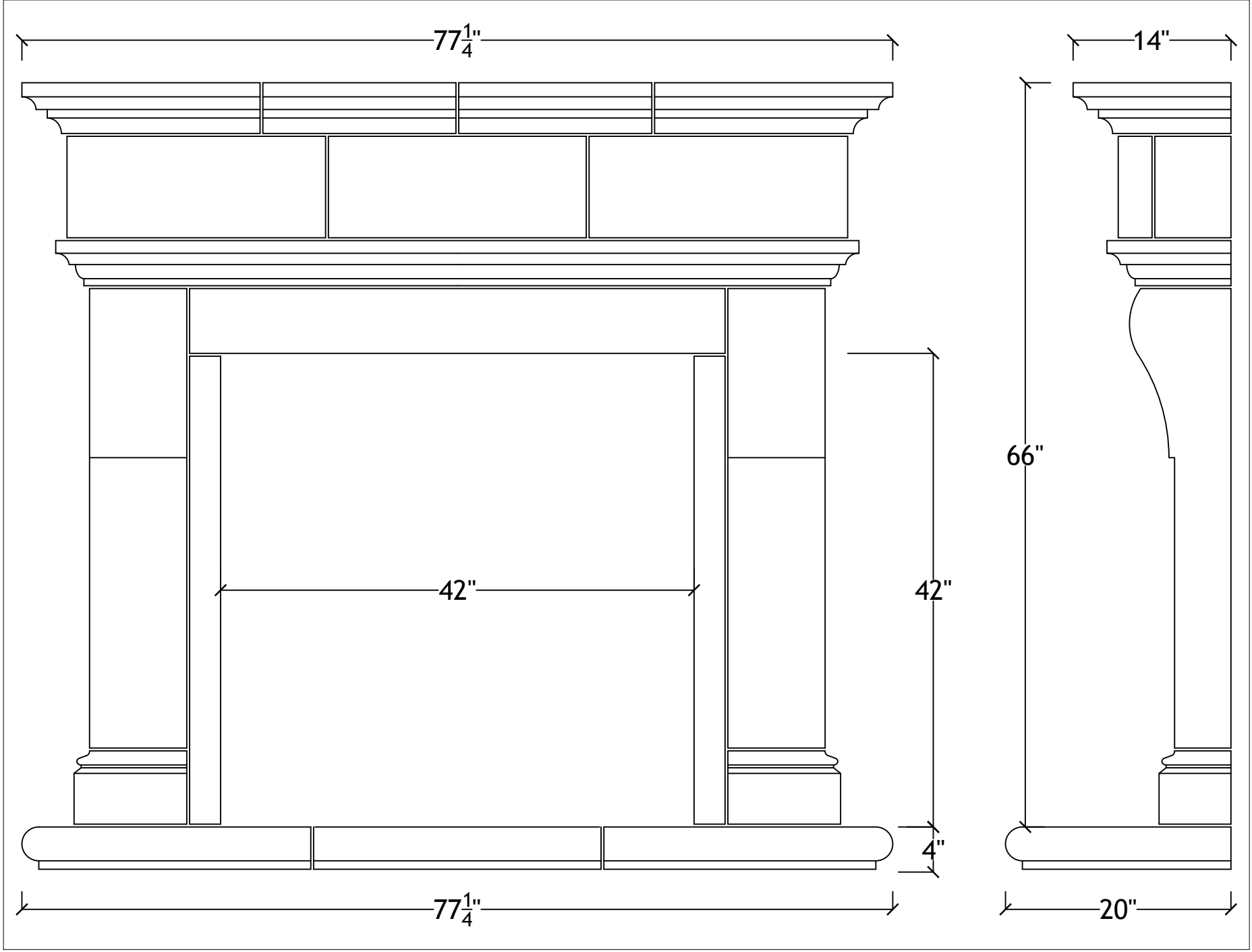
42" Cambridge with bullnosed hearth
