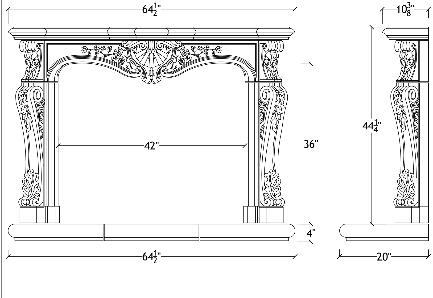
42" Calais with bullnosed hearth
