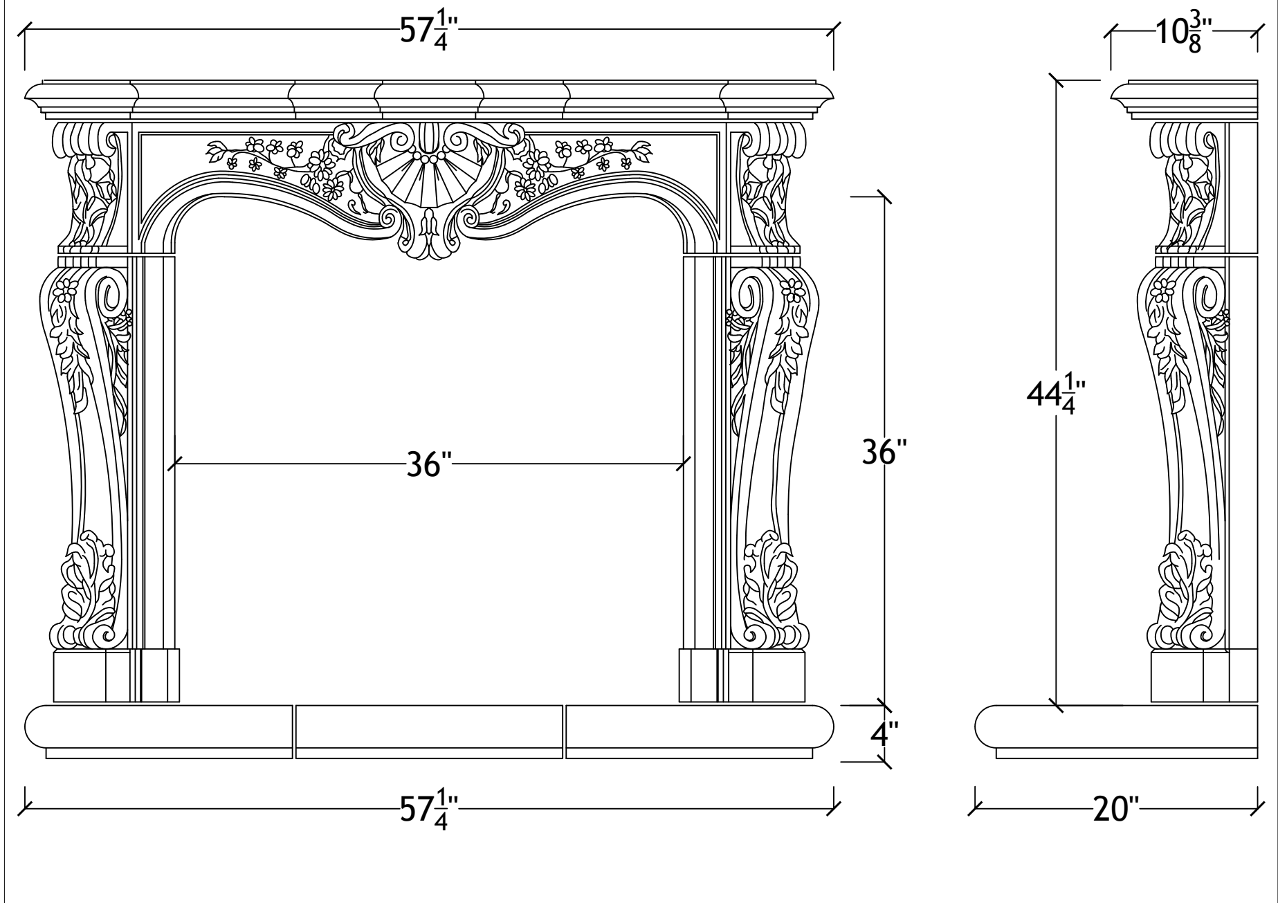
36" Calais with bullnosed hearth
