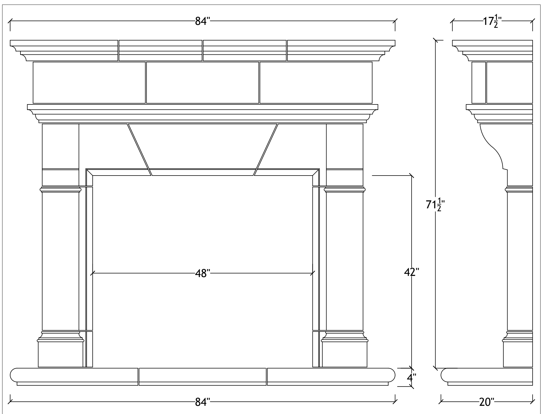
48" Brunswick with bullnosed hearth
