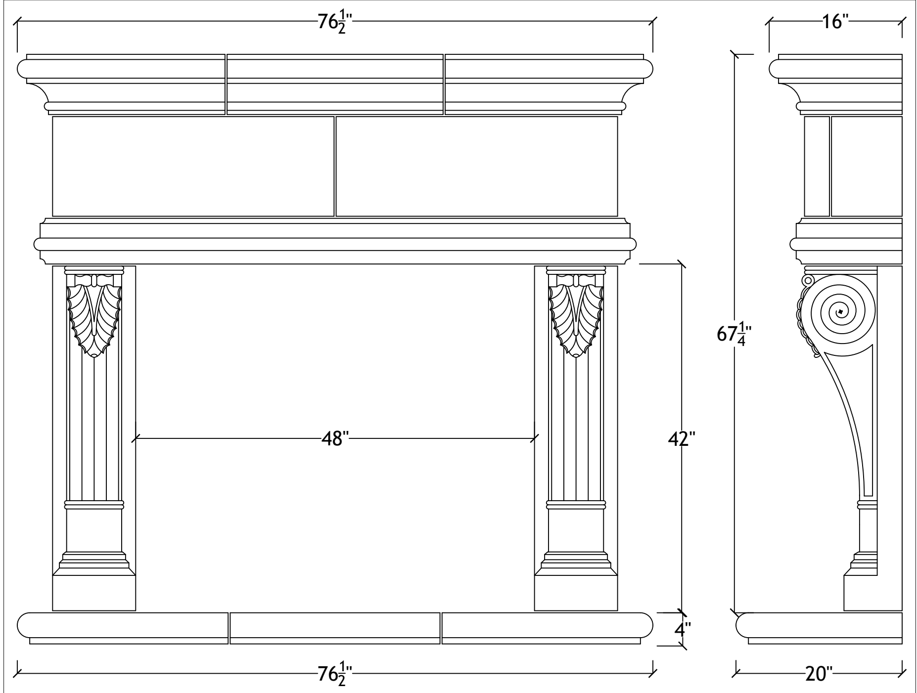
48" Berkley with bullnosed hearth
