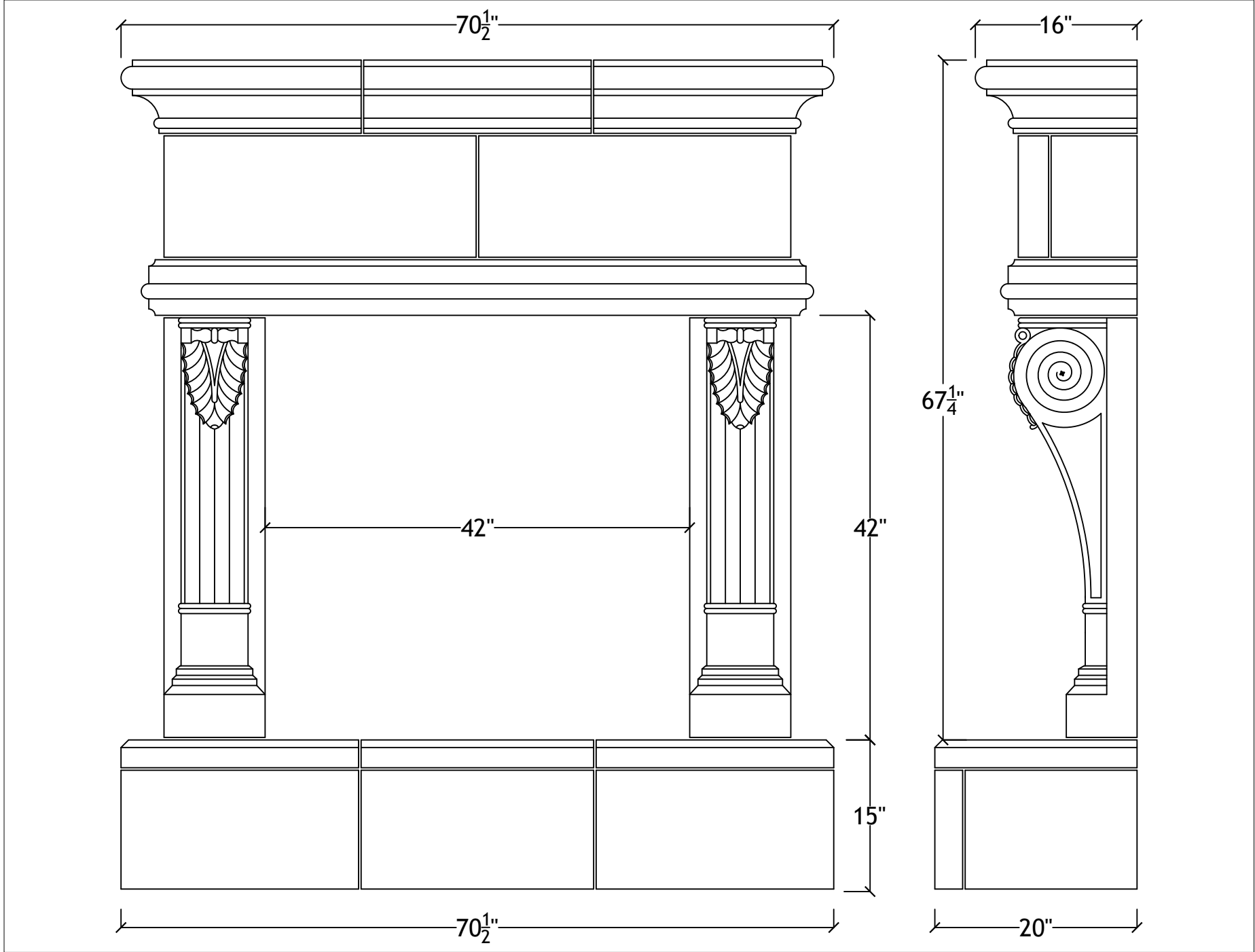
42" Berkley with raised hearth
