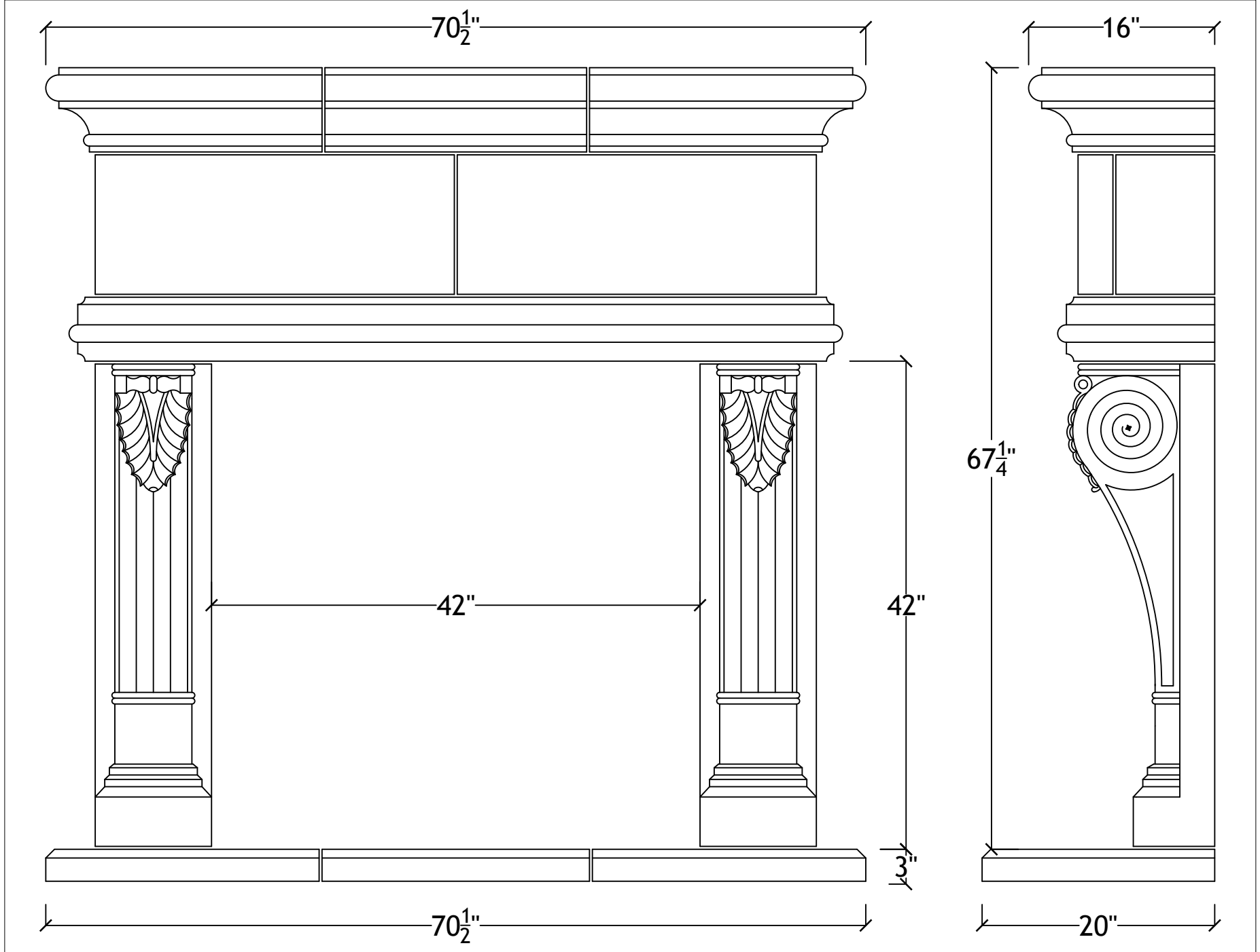
42" Berkley with hearth
