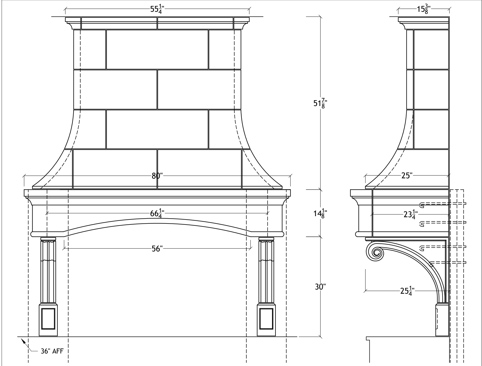
60" Bentwood Range Hood for 11' ceiling
