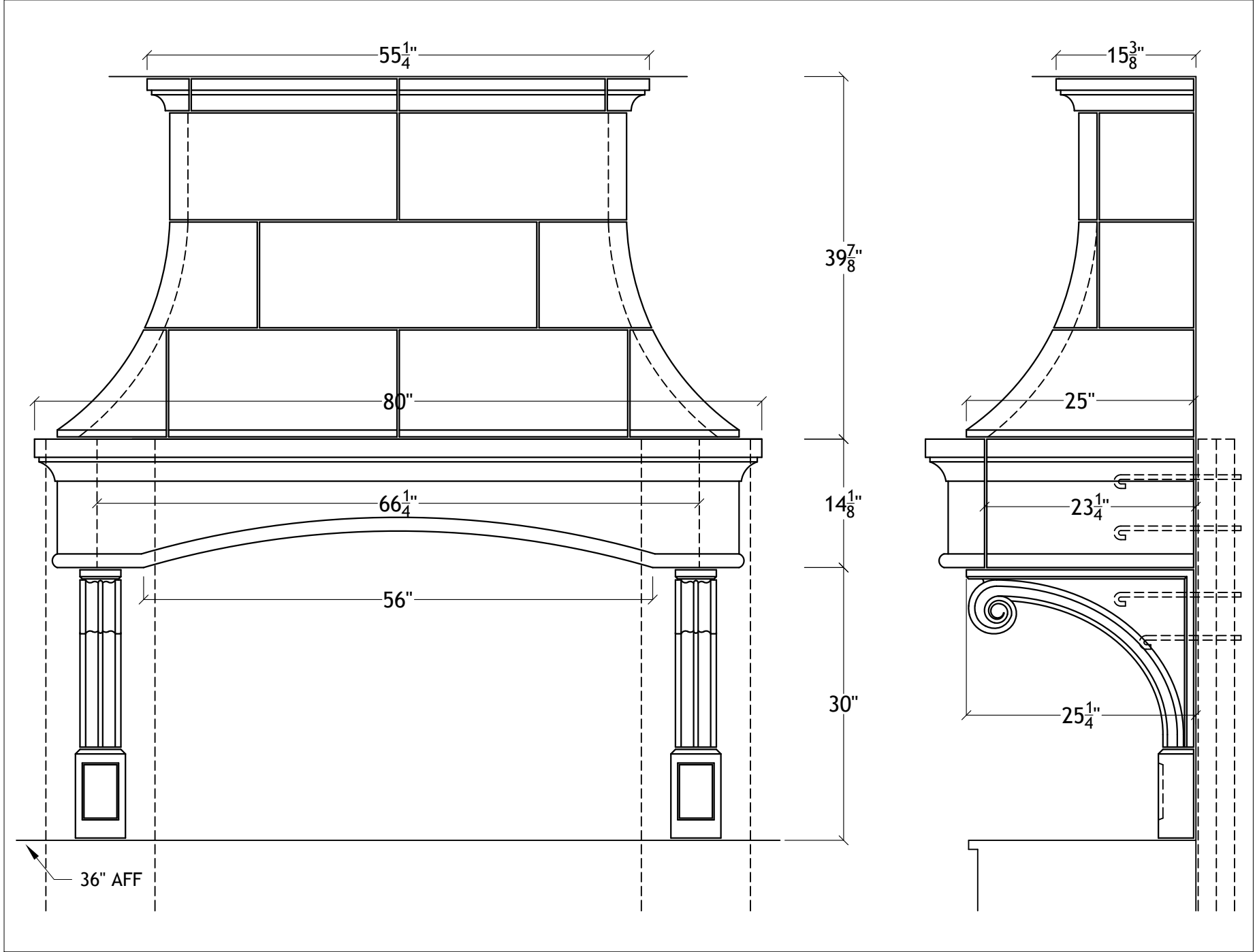
60" Bentwood Range Hood for 10' ceiling
