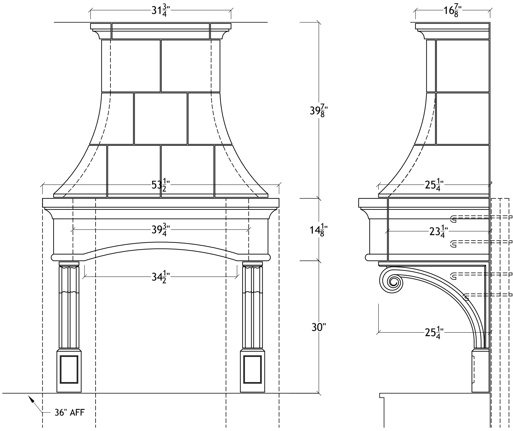
36" Bentwood Range Hood for 10' ceiling
