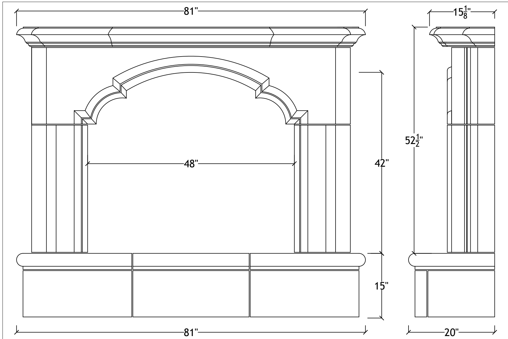
48" Avondale with raised bullnosed hearth
