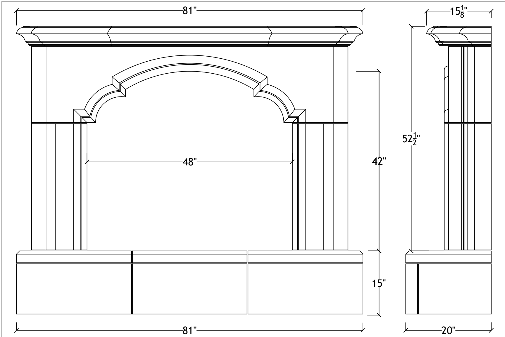
48" Avondale with raised hearth
