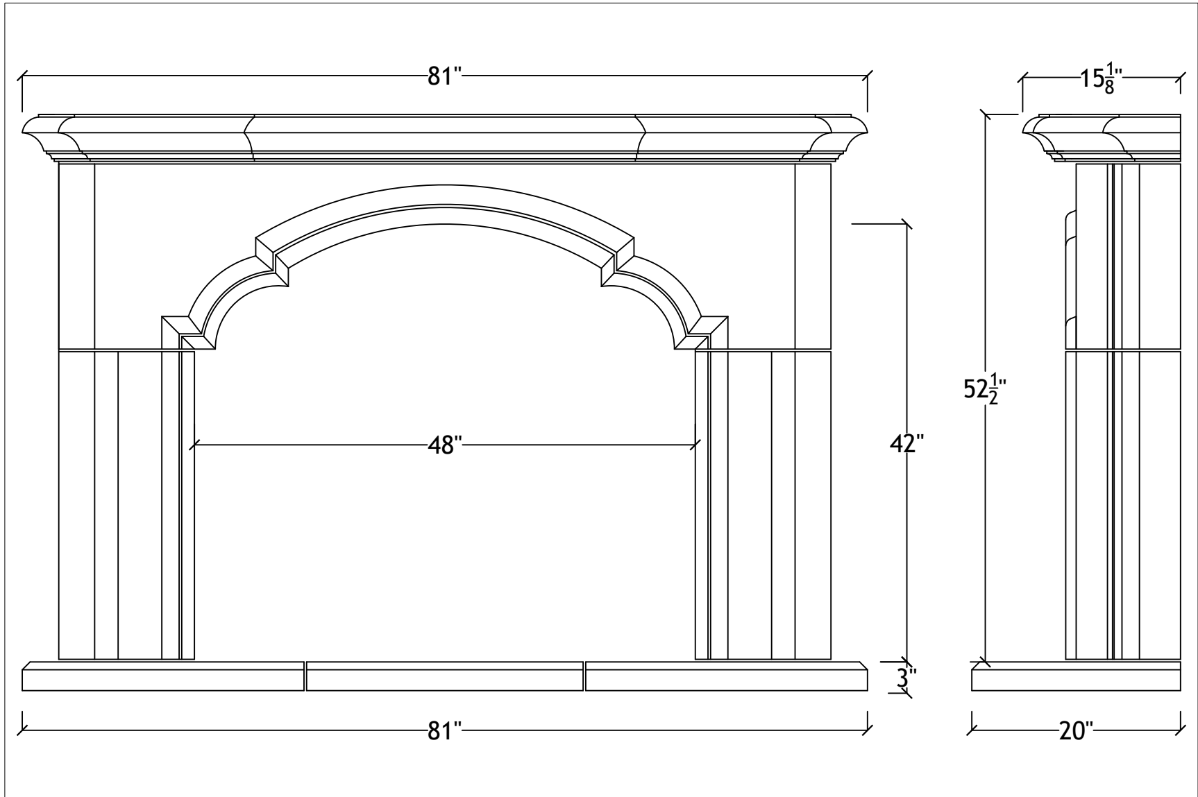
48" Avondale with hearth
