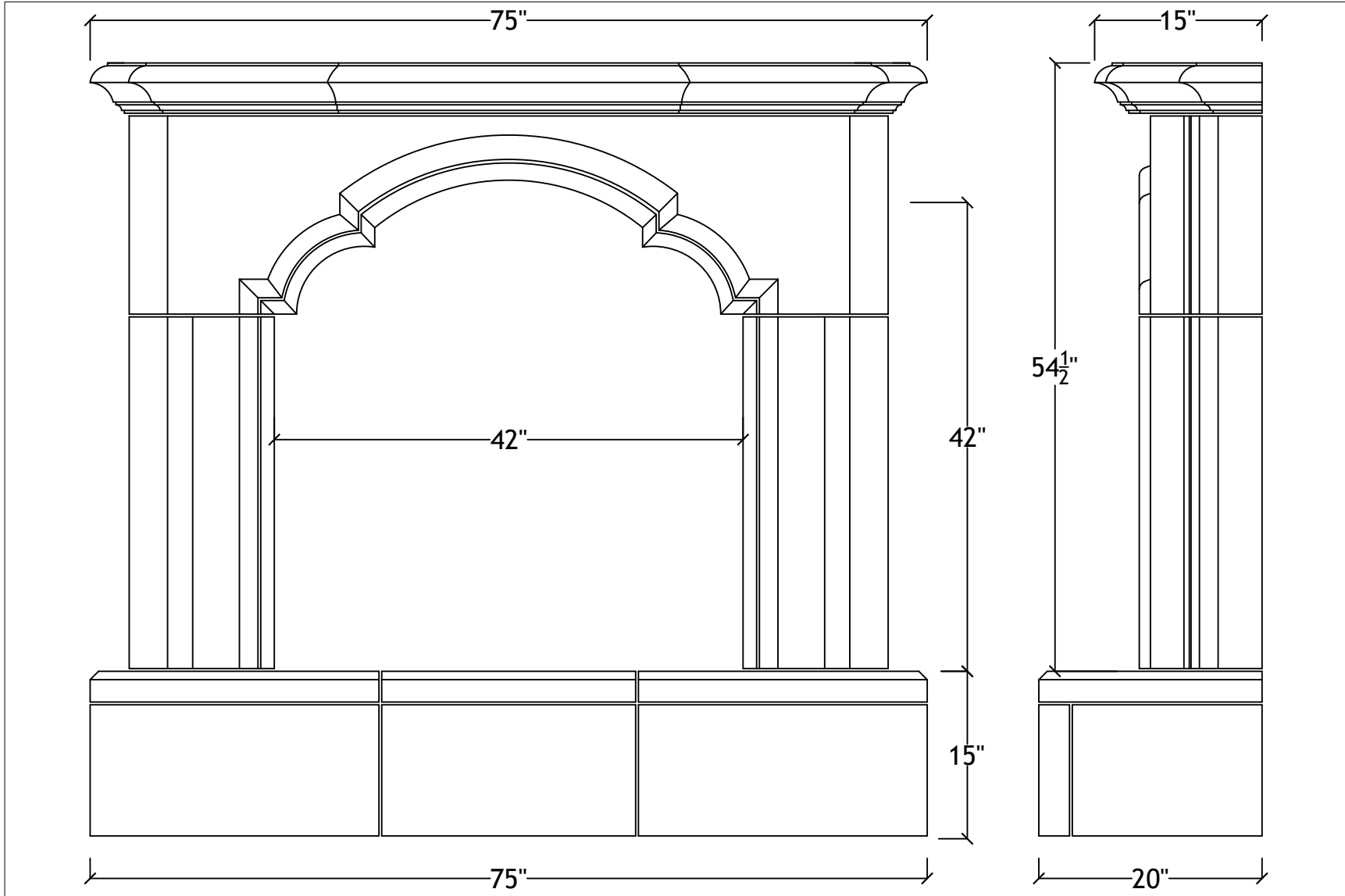
42" Avondale with raised hearth
