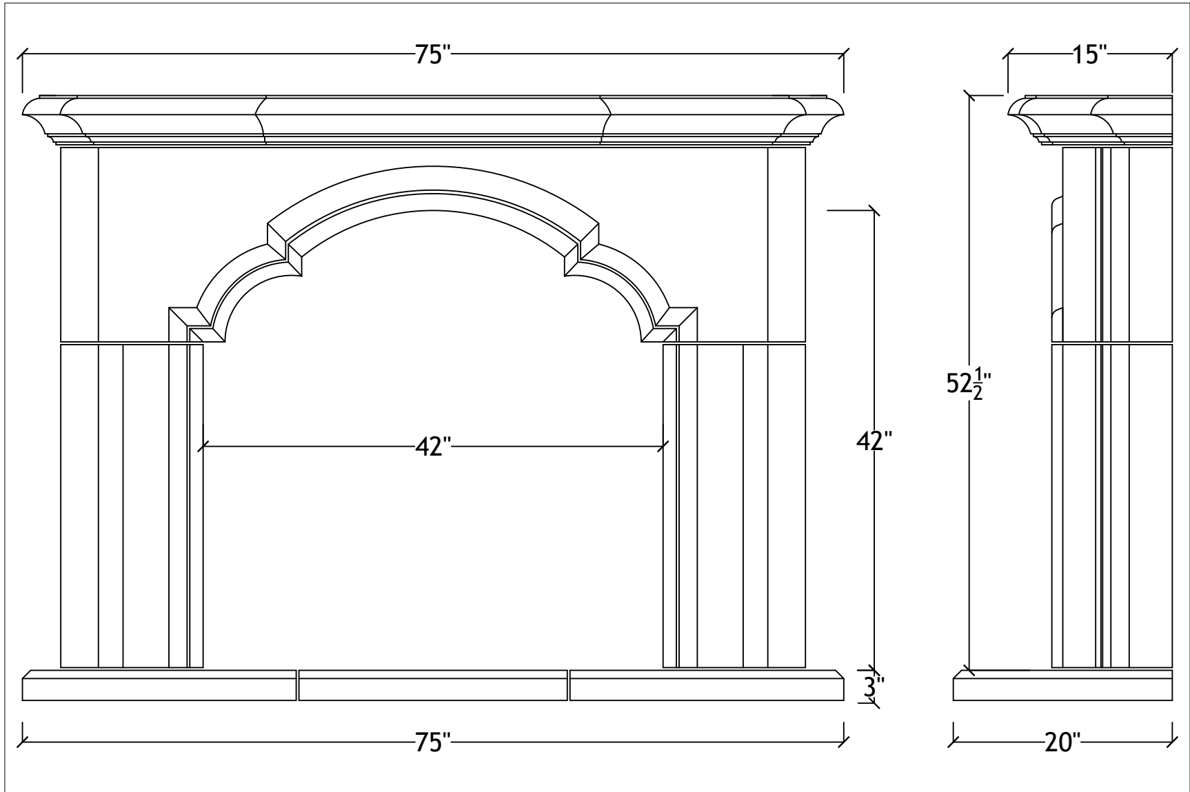
42" Avondale with hearth
