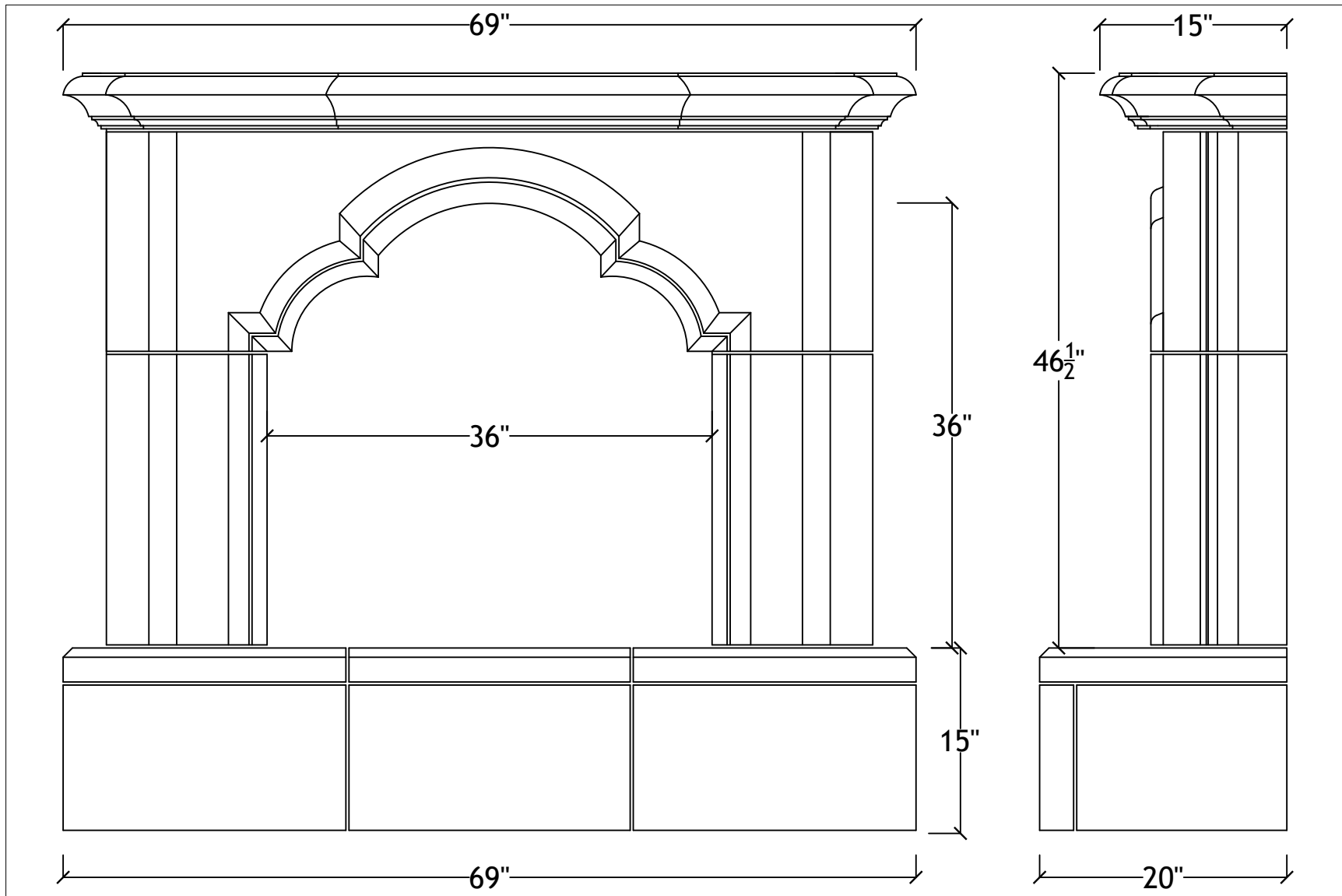
36" Avondale with raised hearth
