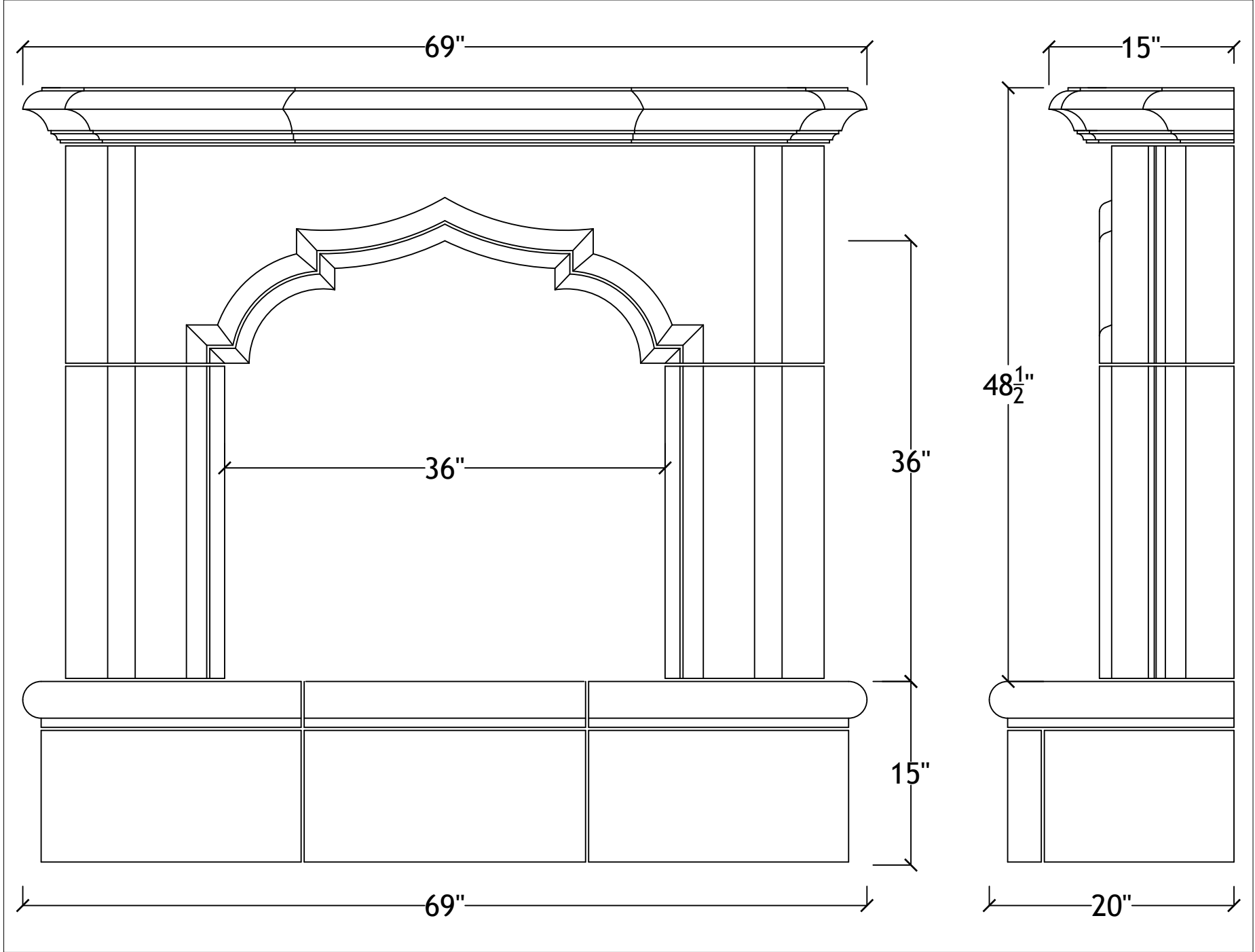
36" Avalon with raised bullnosed hearth
